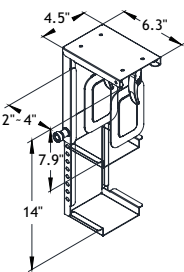
Miniature CPU Holder
