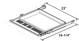
Sliding Drawer
