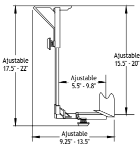
CPU Holder
