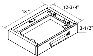
Drawer
