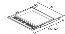
Sliding Drawer
