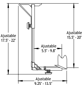
CPU Holder
